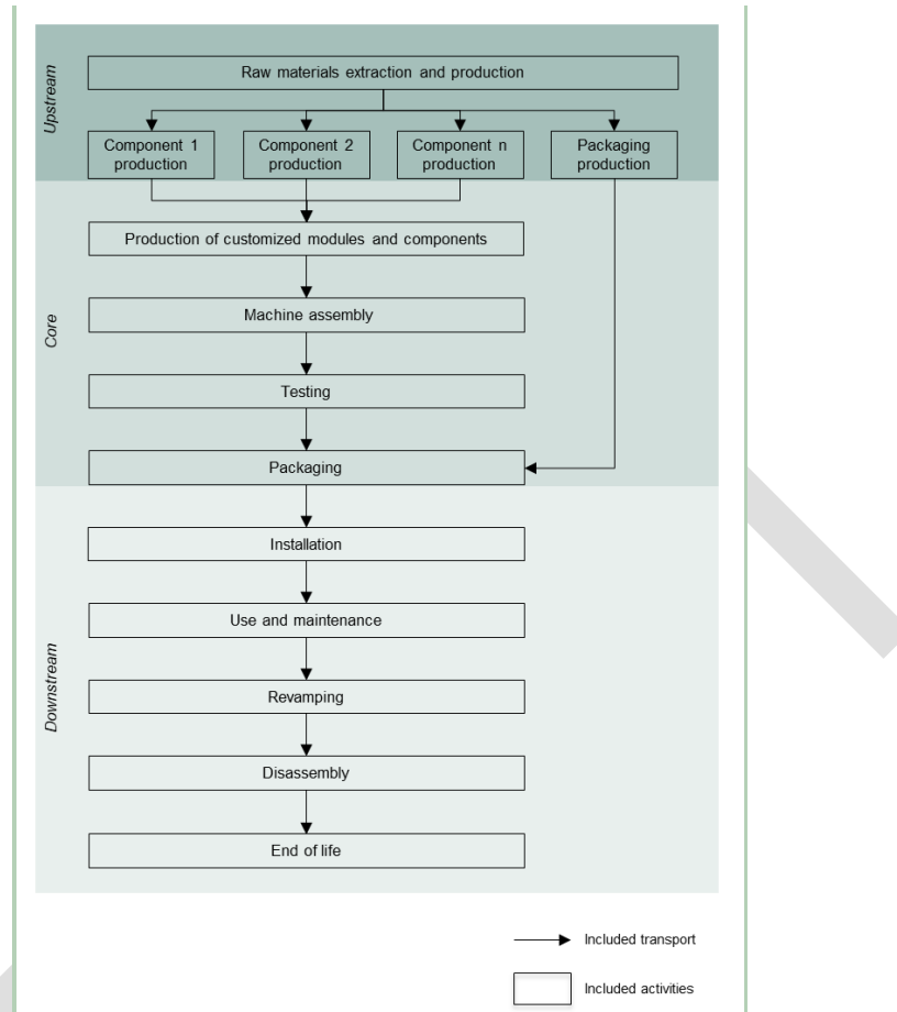
Figure 2 System diagram illustrating the processes that shall be included in the product system, divided into upstream, core and downstream processes. The illustration of processes to include may not be exhaustive.
