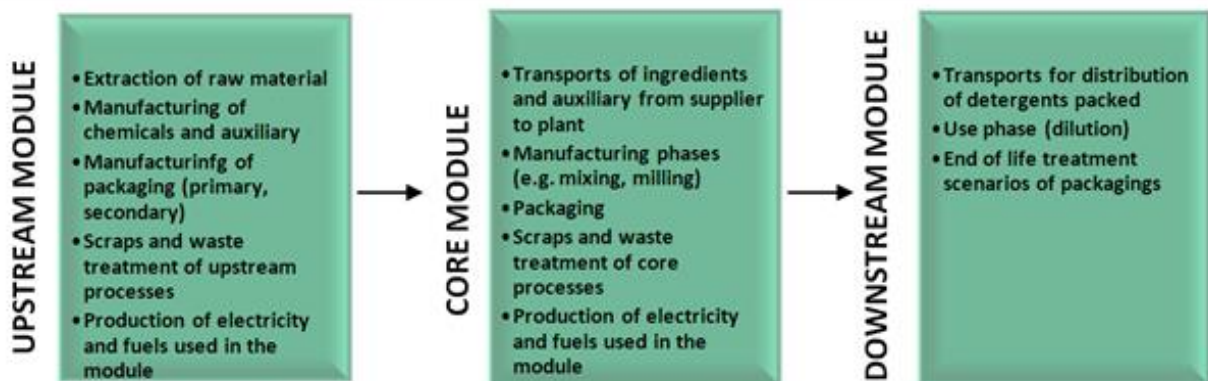
Figure 2 System diagram illustrating the processes that are included in the product system, divided into upstream, core and downstream processes. The list of processes to include may not be exhaustive.
