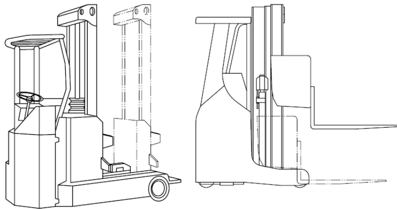
Figure 4. Reach truck
