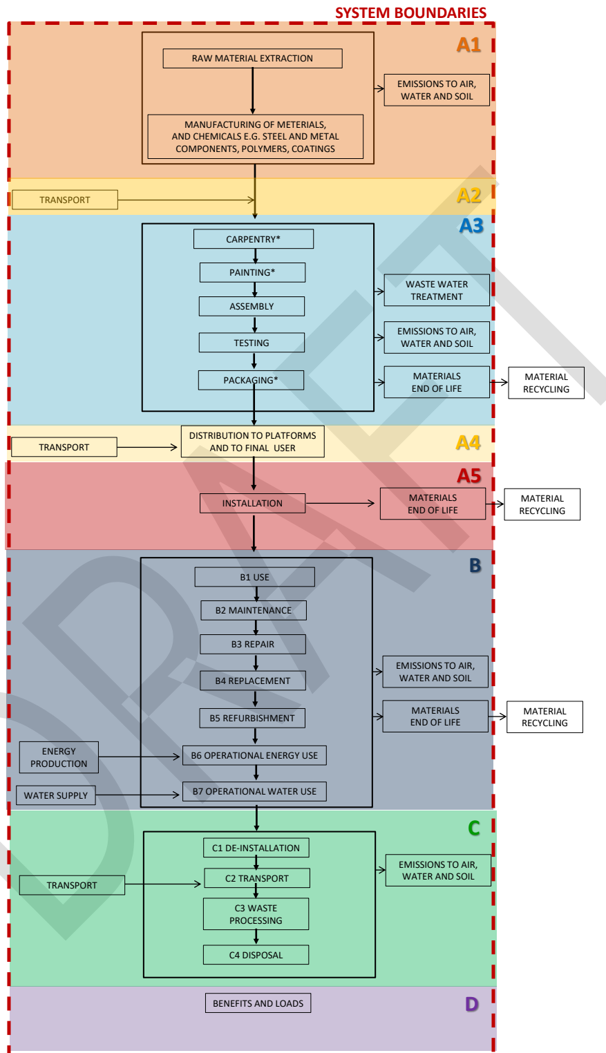
Figure 2. Process flow diagram illustrating the processes that shall be included in the product system, divided into the life-cycle stages. The illustration of processes to include may not be exhaustive. *=operations that can be internally or externally
