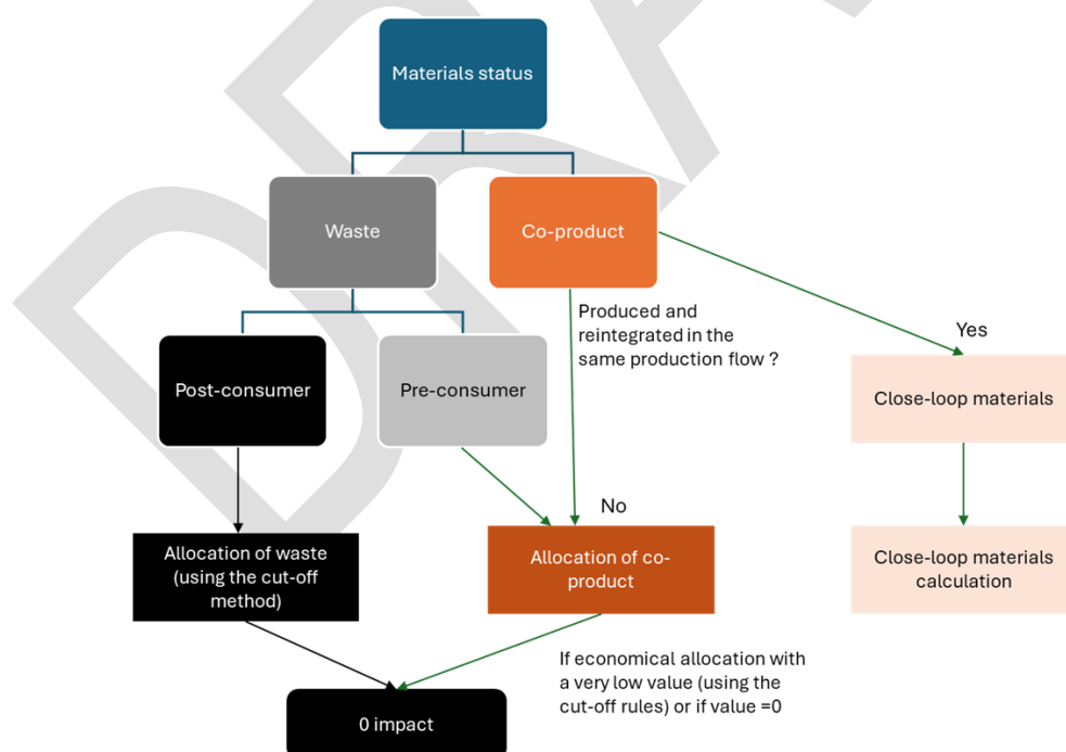
Figure 4. Allocation decision tree for input flows
