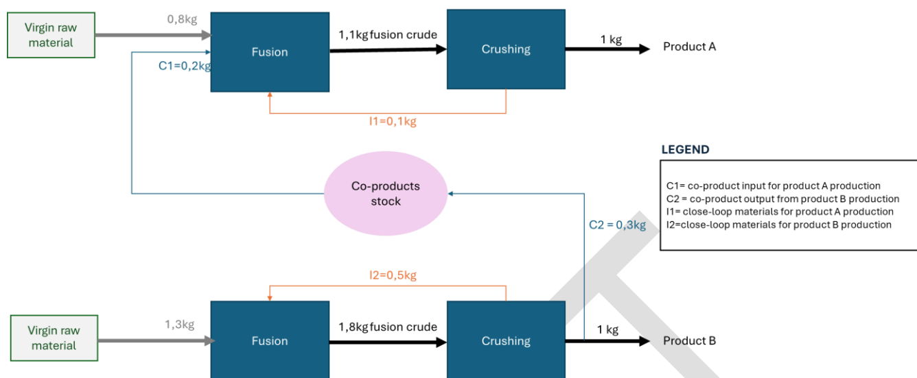
Figure 9 Example 3 flow-chart after classification of the flows
