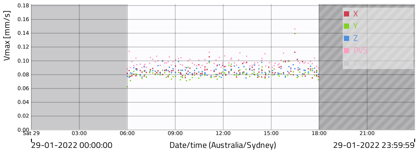
Peak vibration velocity/frequency
