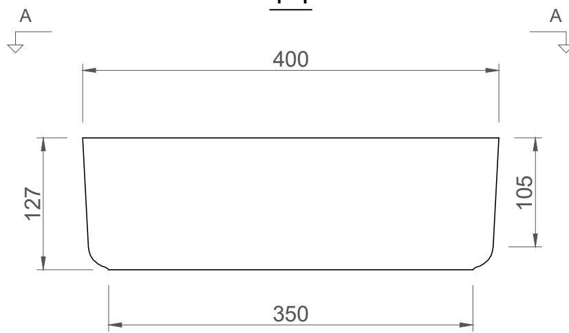
FRONT VIEW 1-1
