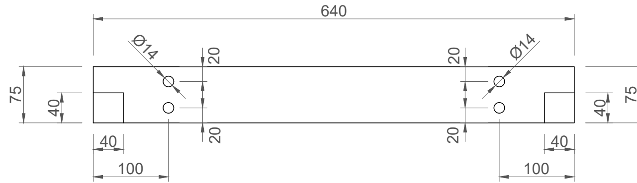
FRONT ELEVATION
