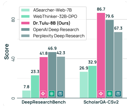
Figure 1 DR Tulu-8B matches or exceeds proprietary deep research models (gray) and outperforms open-source models (green) on deep-research benchmarks.
