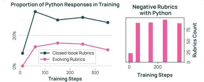
Figure 4 Effect of negative evolving rubrics. Over training, negative evolving rubrics emerge that penalize undesirable behavior such as responding in Python (right), resulting in a reduction in undesirable behaviors over the course of training compared to using a static closed-book rubric that does not specify such undesirable behavior (left).
