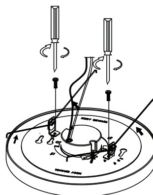
5" Housing Position
