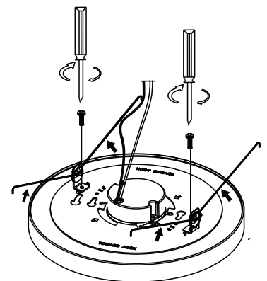
6" Housing Position
