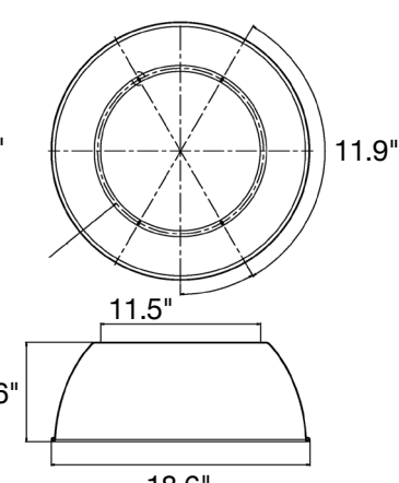
Aluminum Reflector
