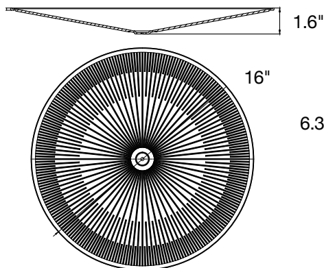
Acrylic Bottom Cover (90°)
