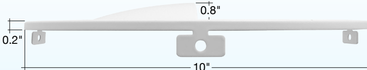
CMD-8-WASH-WH
