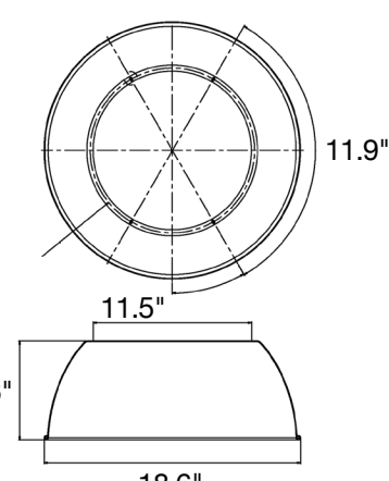
Aluminum Reflector
