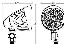
1/2" Knuckle Mount
