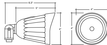
1/2" Knuckle Mount
