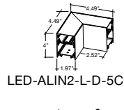
LED-ALIN2-120L-D-5CCT-WH
