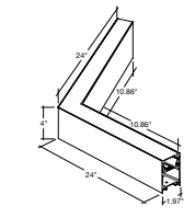
LED-ALIN2-12X12-120L-3P25
