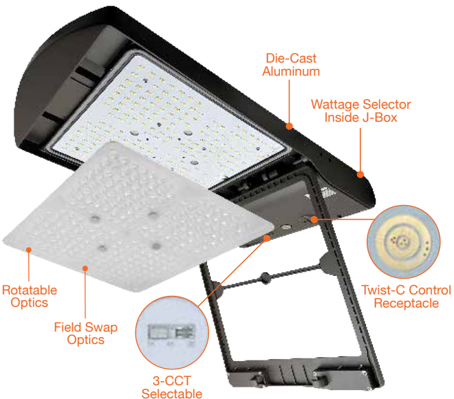
Toolless Access to Optic Lens Toolless Access to Driver
