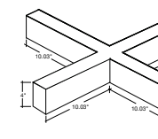
LED-ALIN2-22X22-X-3P50
