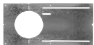
C6-JBX-RI 6" Rough In Plate 8 1/2" x 17 1/4"
