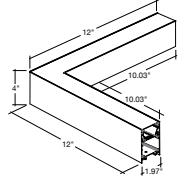
LED-ALIN2-12X12-L-3P25
