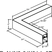
LED-ALIN2-24X24-L-3P50
