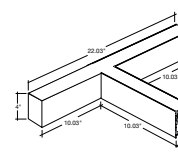
LED-ALIN2-22X10-T-3P36
