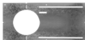
C6-JBX-RI 6" Rough In Plate 8 1/2" x 17 1/4"
