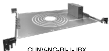
CUNV-NC-RI-J-JBX 21.2" W x 12" D x 1.6" H (Assembly Required)
