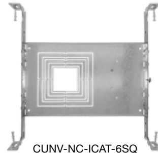
CUNV-NC-ICAT-6SQ Universal Construction Plate 14" x 13.75"
