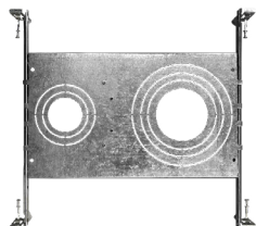
CUNV-NC-ICAT-7H Universal Pre-Mounting Plate 13 7/8" x 15 1/8"
