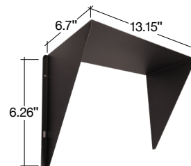
ARL3-240-300W-HSS-BZ
