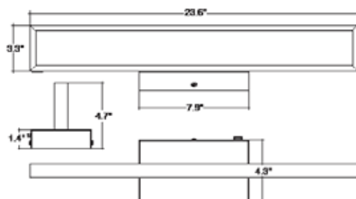
Indirect Light (Top View)
