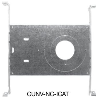
CUNV-NC-ICAT Universal Pre-Mounting Plate 5 3/10" x 14 1/2"
