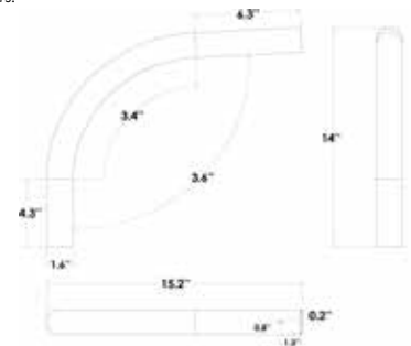
Tenon Bracket Dimensions
