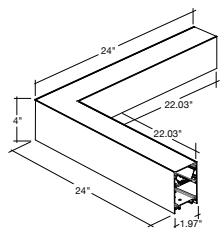
LED-ALIN2-FL-24X24-L-3P50
