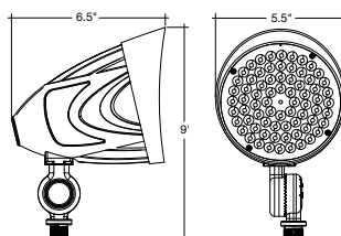
1/2" Knuckle Mount
