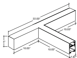
LED-ALIN2-FL-22X10-T-3P36
