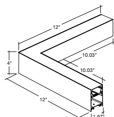
LED-ALIN2-FL-12X12-L-3P25
