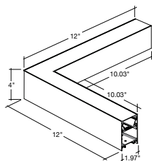
LED-ALIN2-FL-12X12-L-3P25
