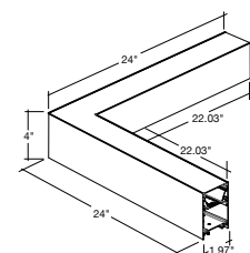
LED-ALIN2-FL-24X24-L-3P50
