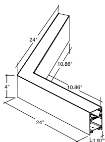
LED-ALIN2-FL-12X12-120L-3P25
