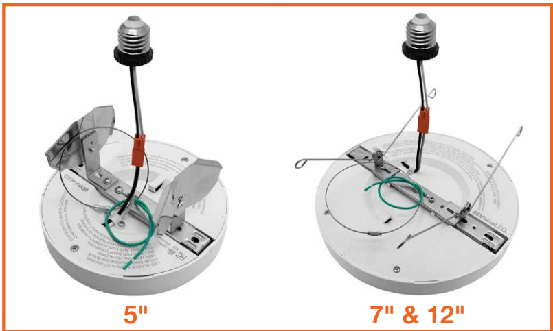
RETROFIT KIT CAN CONVERTER
