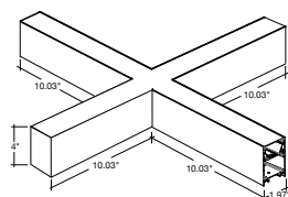
LED-ALIN2-FL-22X22-X-3P50
