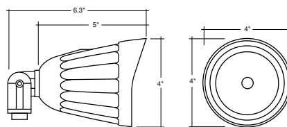
1/2" Knuckle Mount
