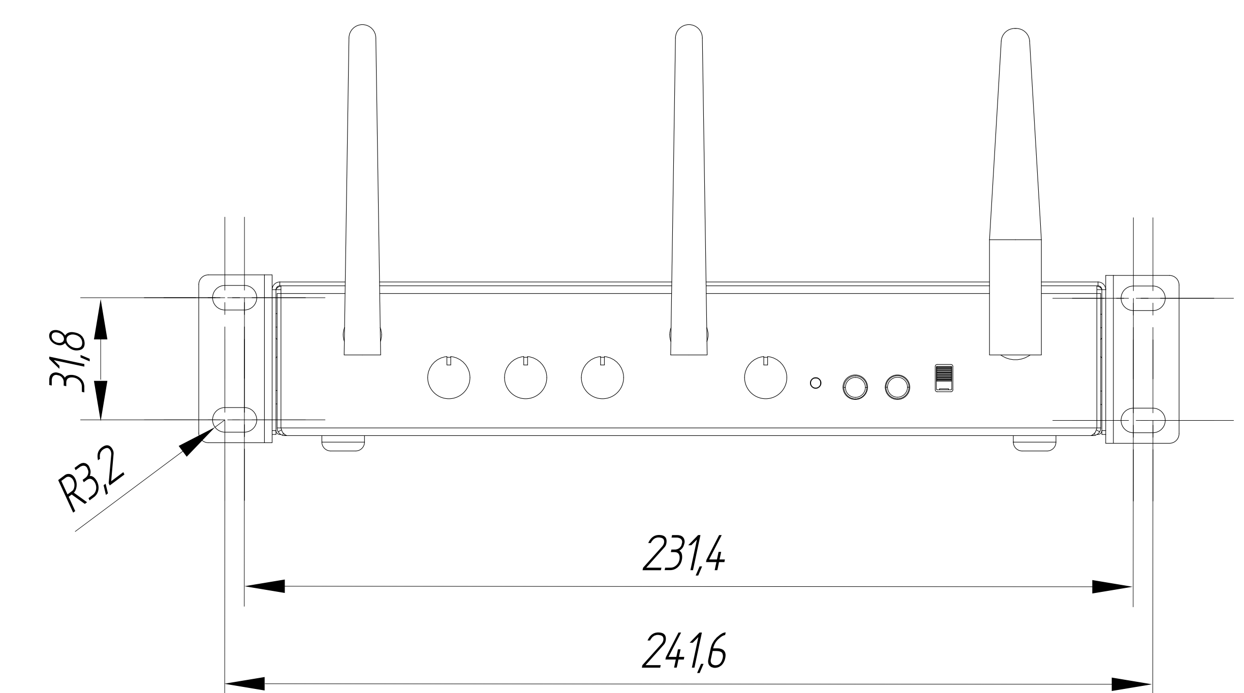
FRONTAL FIXING ACCESSORY (OPTION 2)
