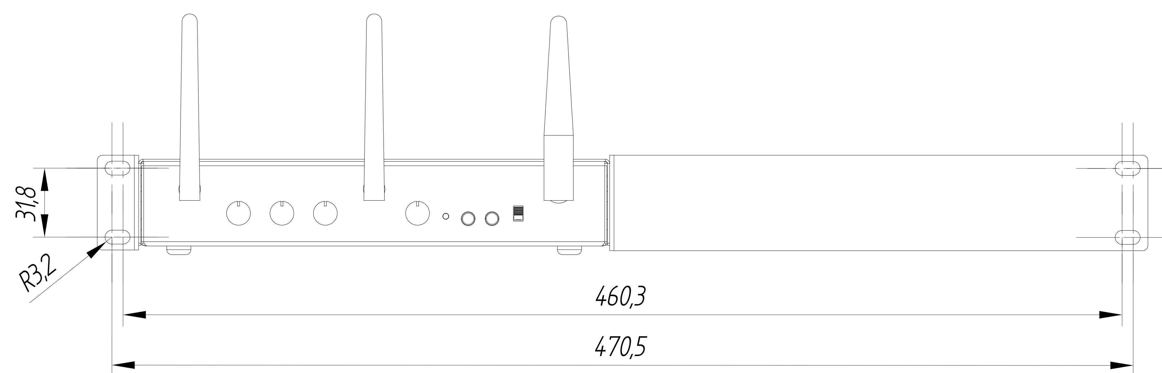
FRONTAL FIXING ACCESSORY (OPTION 1)
