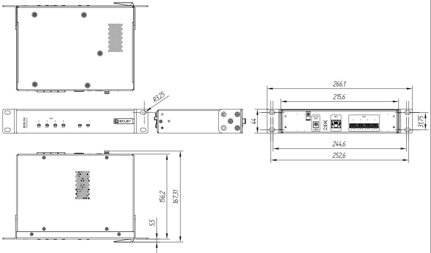
Ecler BOB-04 Mechanical Diagram
