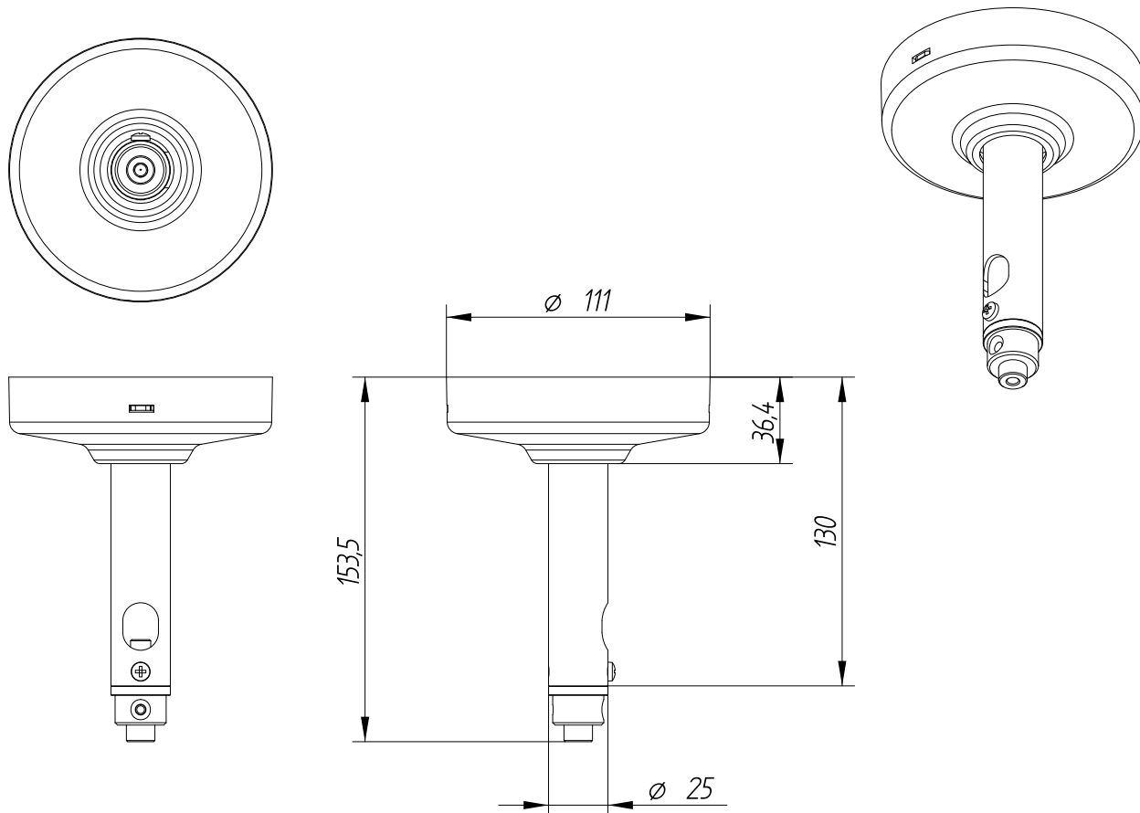
Ecler CEILY Mechanical Diagram
