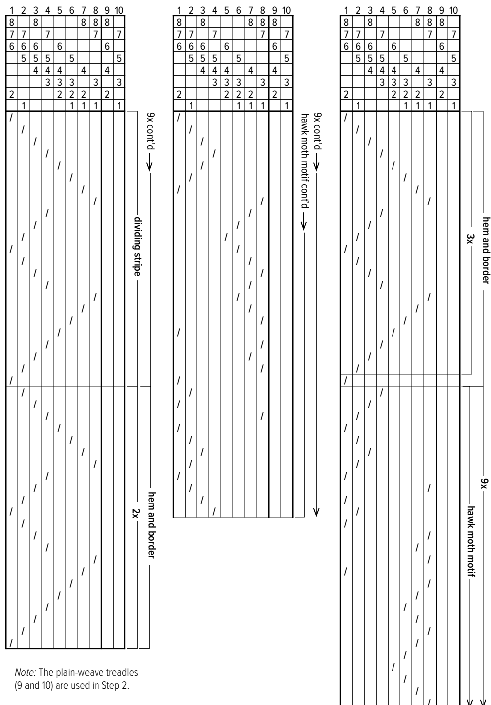
FIGURE 2. DRAFT TREADLING
