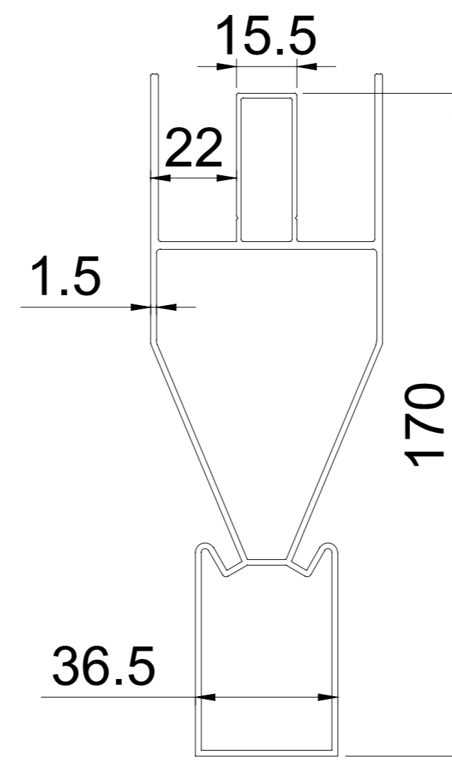
Middle Beam
