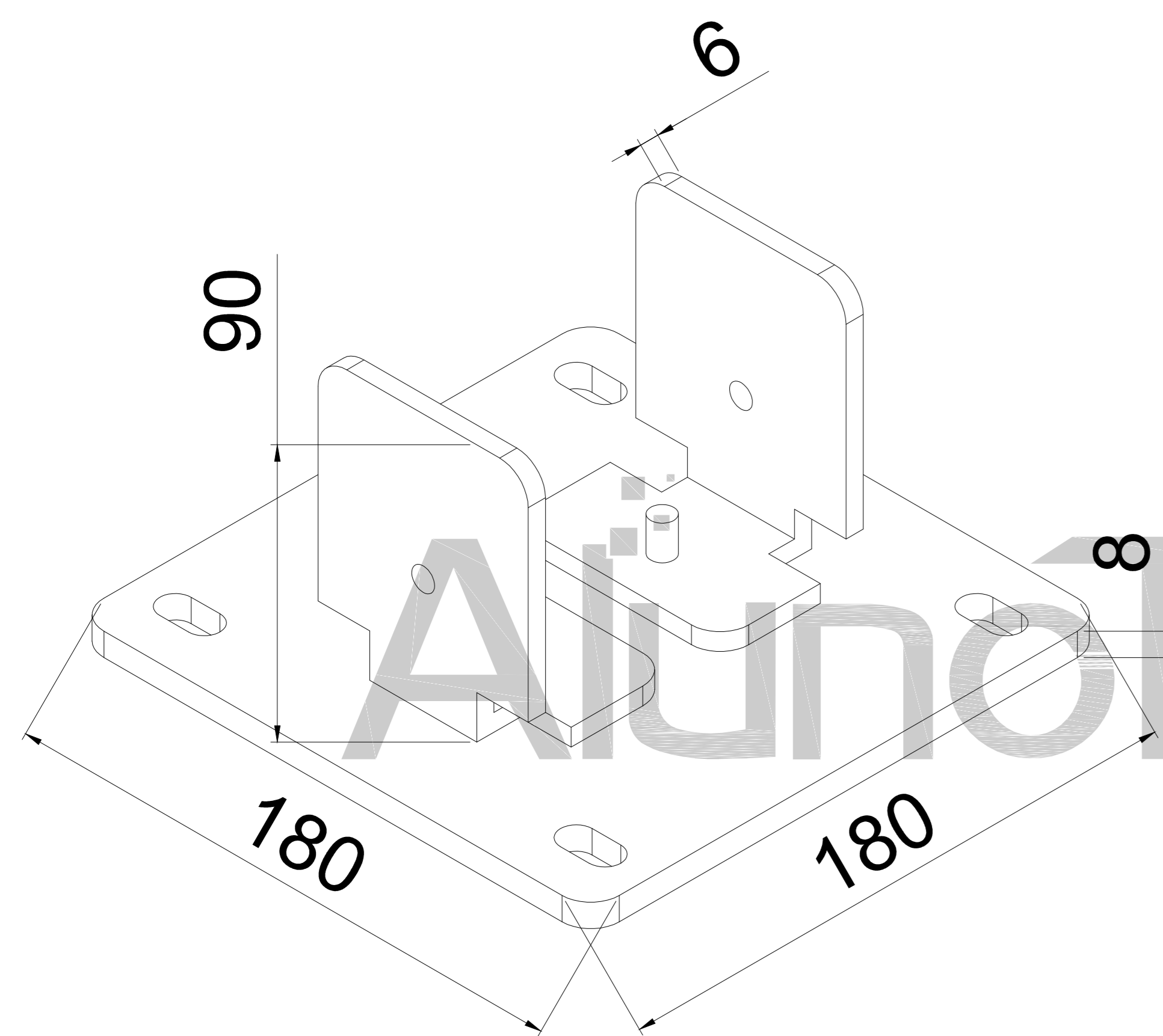
Base Plate
