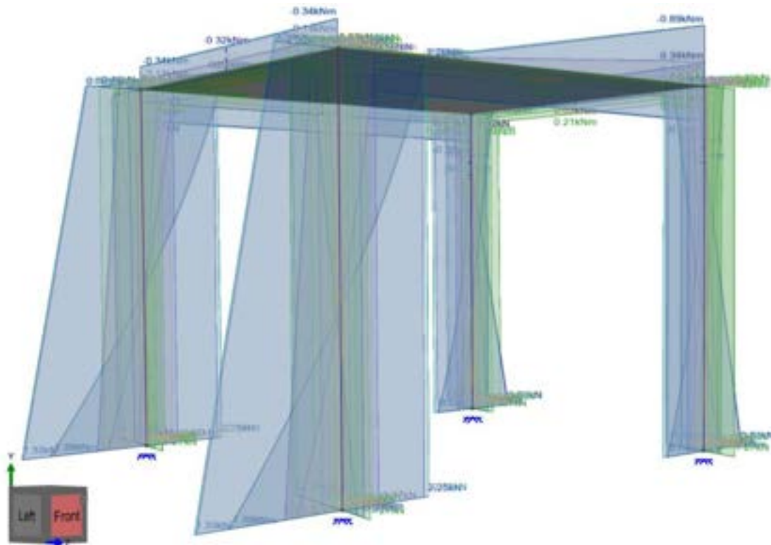
Figure 2 - Reaction Forces & Moments
