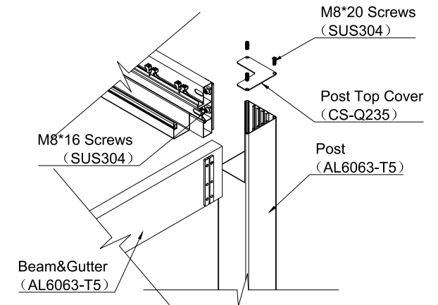
3 5 Connection of Post and Plate base
