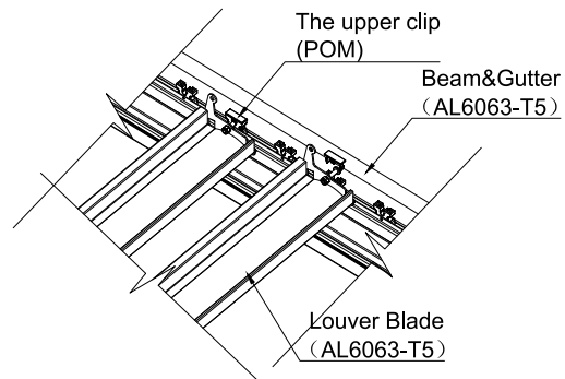
4 5 Connection of blade and beam
