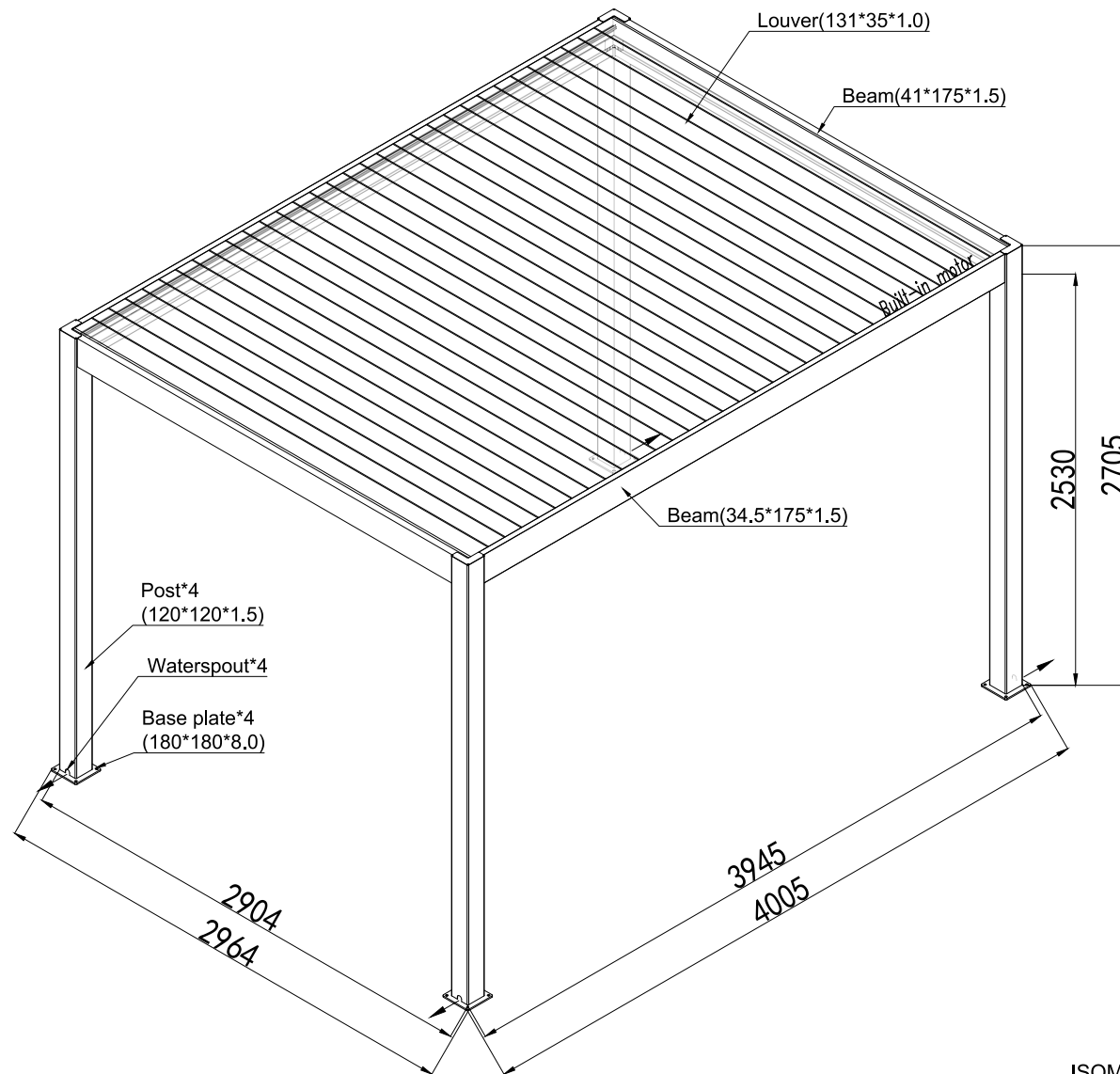
ISOMETRIC VIEW
