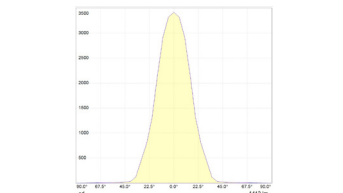
LED Solo Spot Cartesian diagram
