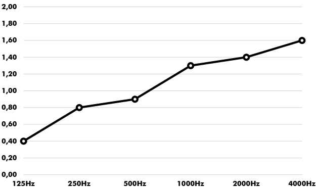
BuzziBurner Ceiling Suspended Equivalent sound absorption area in m² per object
