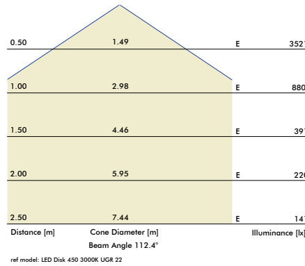
LED Disk Polar curve
