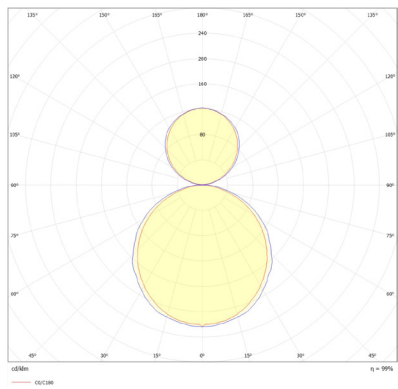
Polar curve
