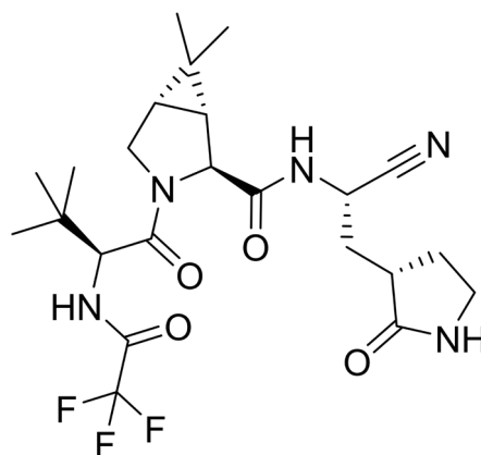
PF-07321332/nirmatrelvir PDB: 7RFS
