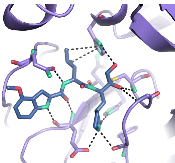
PF-00835231
