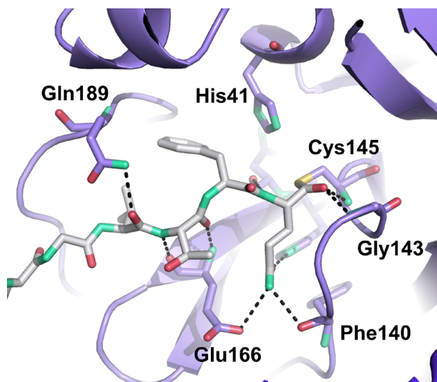
C-term. autopeptide: SGVTFQ 7KHP
