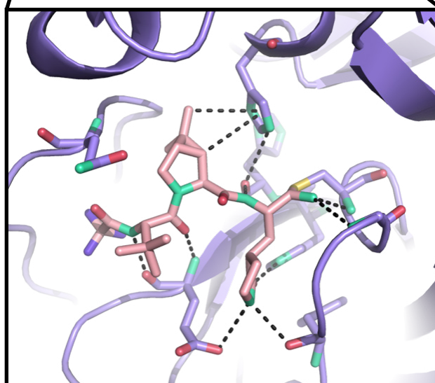
PF-07321332/nirmatrelvir PDB: 7RFS
