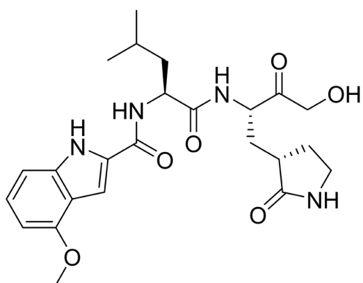
PF-00835231
