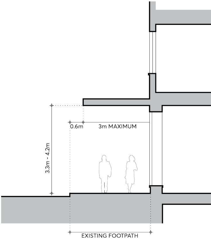
Figure 9.10.14.3 – Detailed Section through Macquarie Street
