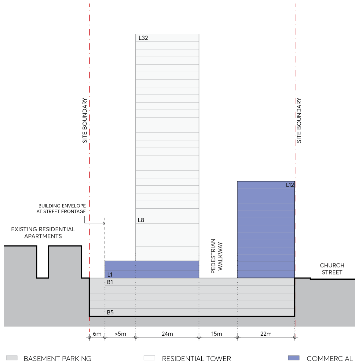
Figure 9.10.2.4 – Building Form Control Section (Northern Side)
