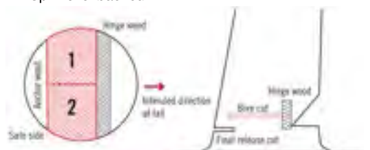
Split level backcut
