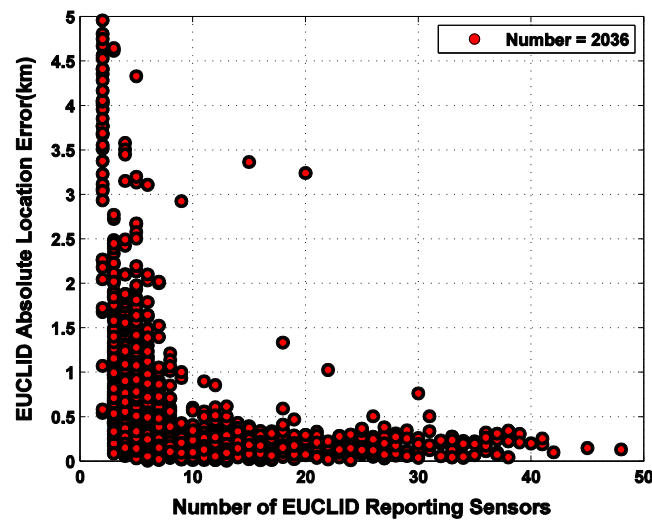
Figure 11. EUCLID absolute location error versus the number of EUCLID reporting sensors.
