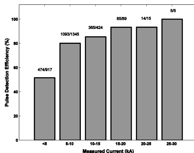
Figure 5. EUCLID detection efficiency as a function of pulse peak current measured at Sântis (the bin size of 5 kA) for upward negative events.
