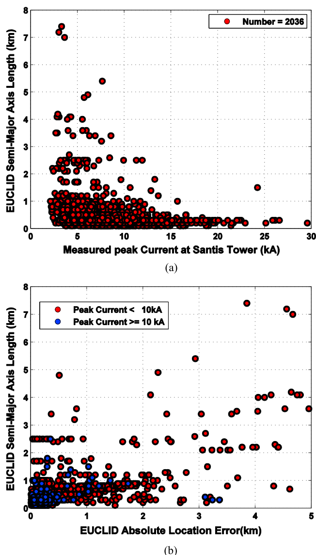
Figure 12. (a) EUCLID semimajor axis length of the 50% confidence ellipse versus peak current value of upward negative pulses measured at the S antis Tower and (b) EUCLID semimajor axis length of the 50% confidence ellipse versus absolute location error of upward negative pulses.
