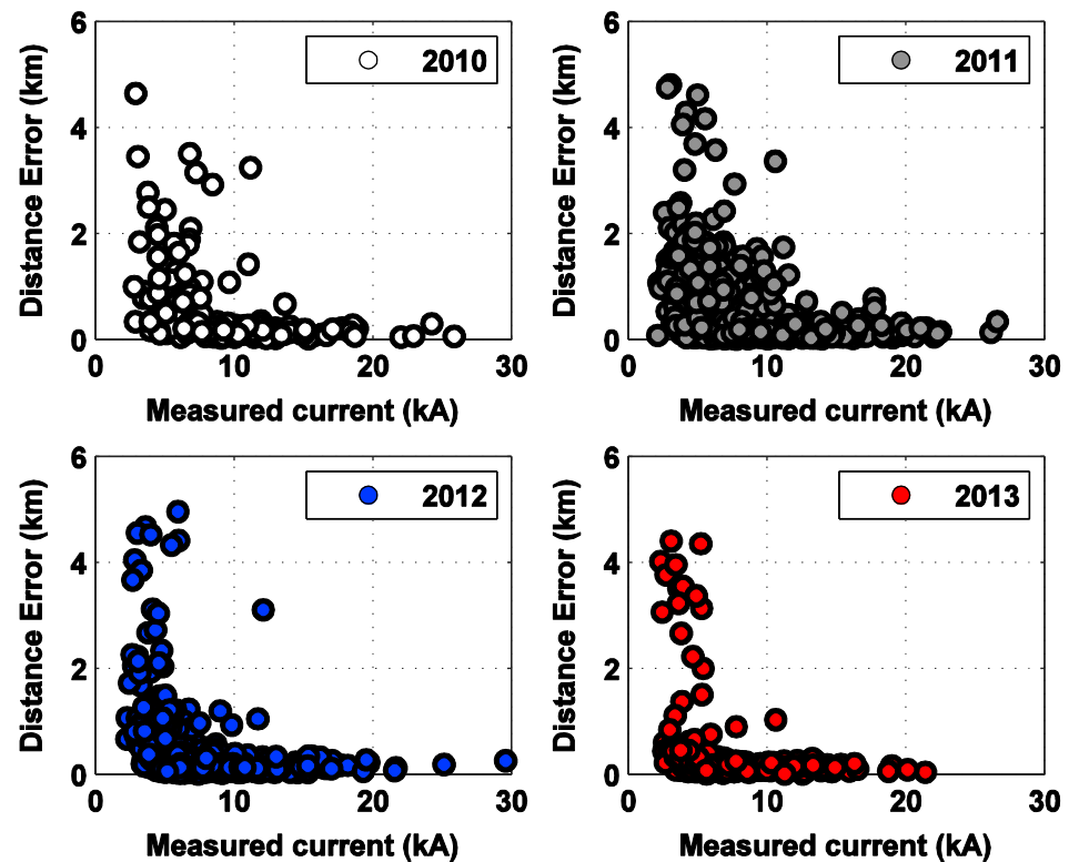
Figure 10. EUCLID absolute location error versus Sântis Tower measured peak current for pulses of upward negative events. Data are presented in different plots and different colors are associated with each of the four years of considered in this study.
