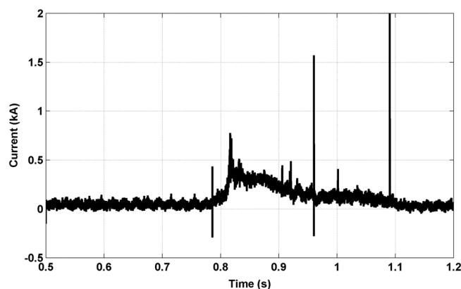
Figure 3. Measured current waveform associated with an upward negative flash recorded on 18:40:15, 25 August 2012. The current is characterized by a low amplitude ICC and ICC pulses with no return strokes.
