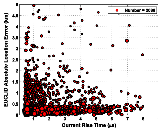
Figure 9. EUCLID absolute location error versus measured 10–90% current rise time for upward negative pulses. The radius of each circle is proportional to the current peak value.
