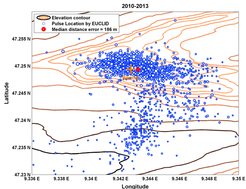
Figure 7. Plot of EUCLID pulse locations for upward negative flashes recorded in the period of analysis. The size of the circles is proportional to the current peak measured at Säntis. The length and width of the shown area are, respectively, 3.34 and 1.06 km.
