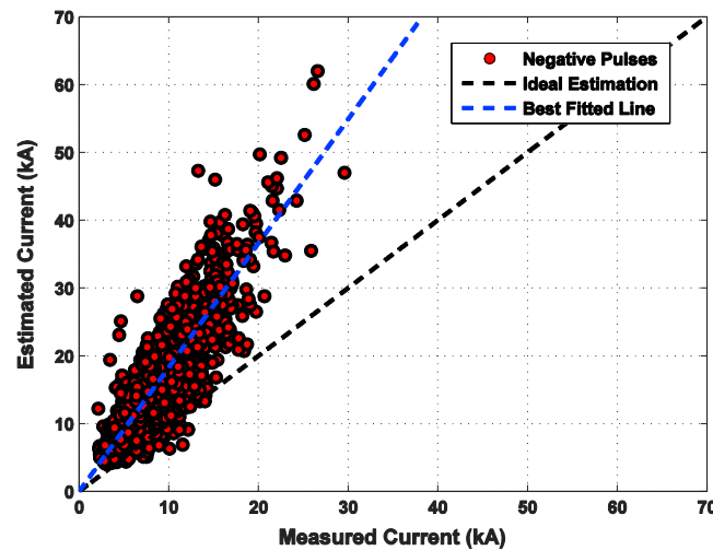
Figure 6. EUCLID peak current estimates versus peak currents directly measured at the Säntis Tower.
