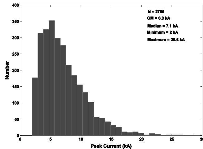
Figure 4. Peak current distribution of pulses associated with upward negative flashes measured at the Sântis Tower.
