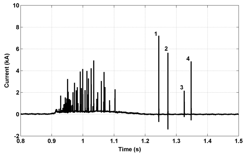
Figure 1. The current waveform associated with an upward negative flash recorded on 14:52:22, 6 August 2012. The initial continuous current (ICC), ICC pulses and 4 return strokes (labeled 1 to 4) can be identified in the waveform.
