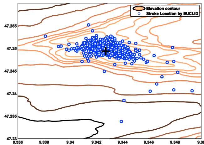
Figure 8. Plot of pulse locations estimated by EUCLID excluding pulses with peak values lower than 10 kA.
