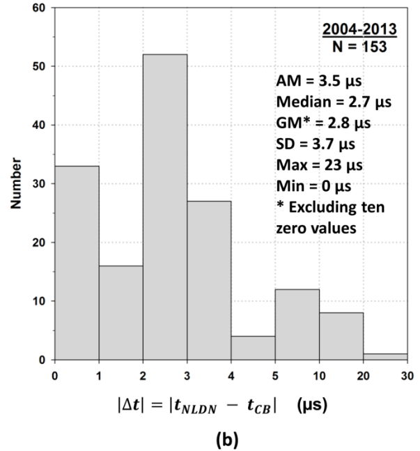
Fig. 9. Histogram of (a) signed and (b) absolute event-time mismatches ( \Delta t = t_{NLDN} - t_{CB} ) for 153 return strokes recorded at Camp Blanding (2004–2013). Statistics given are the arithmetic mean (AM), median, geometric mean (GM), standard deviation (SD), maximum value (Max), and minimum value (Min). N is the sample size.
