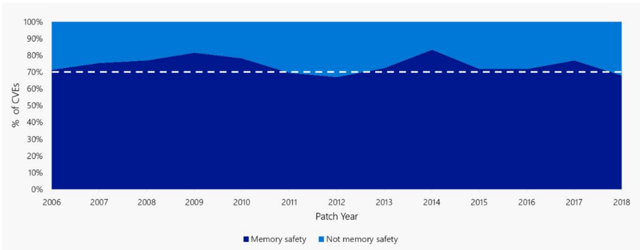
Figure 1: ~70% of the vulnerabilities Microsoft assigns a CVE each year continue to be memory
