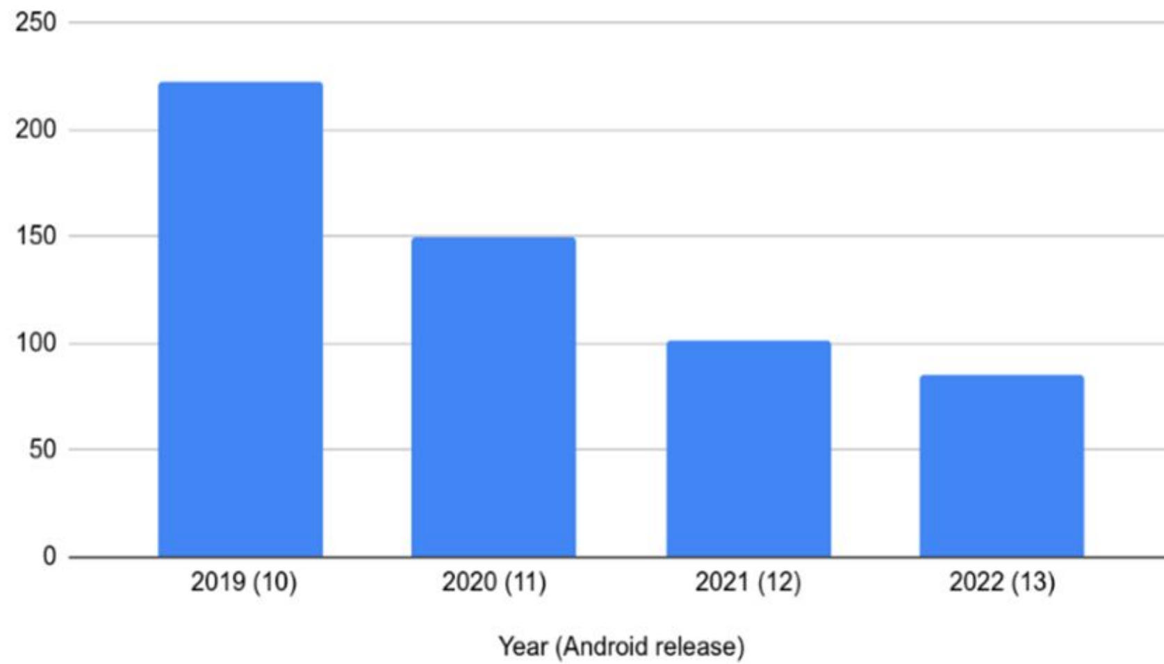
Memory Safety Vulnerabilities Per Year
